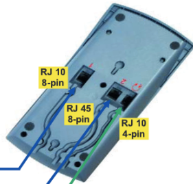
Microphone Loudspeaker Unit Ref. 40.054.301 - bottom side
