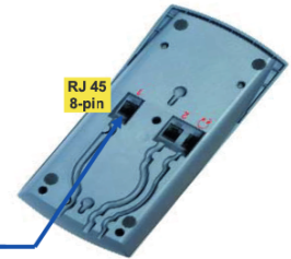
Microphone Loudspeaker Unit Ref. 40.054.301 - bottom side
